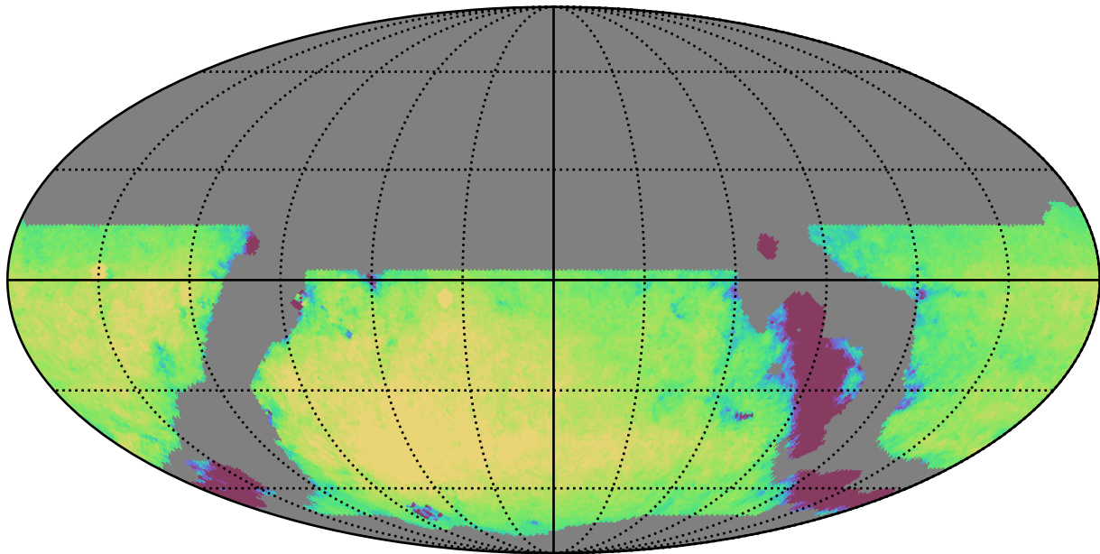
weather_cloudso8v3.4_10yrs WFD g band: Exgal_CoaddM5
