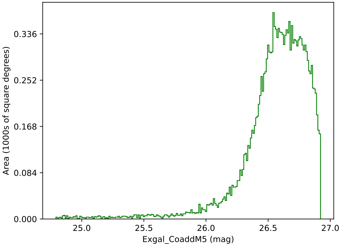
weather_cloudso8v3.4_10yrs WFD g band: Exgal_CoaddM5
