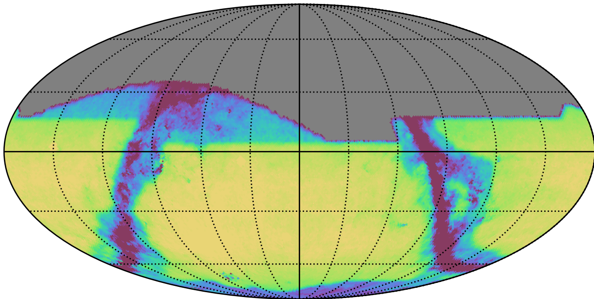
weather_cloudso8v3.4_10yrs All sky z band: Exgal_CoaddM5
