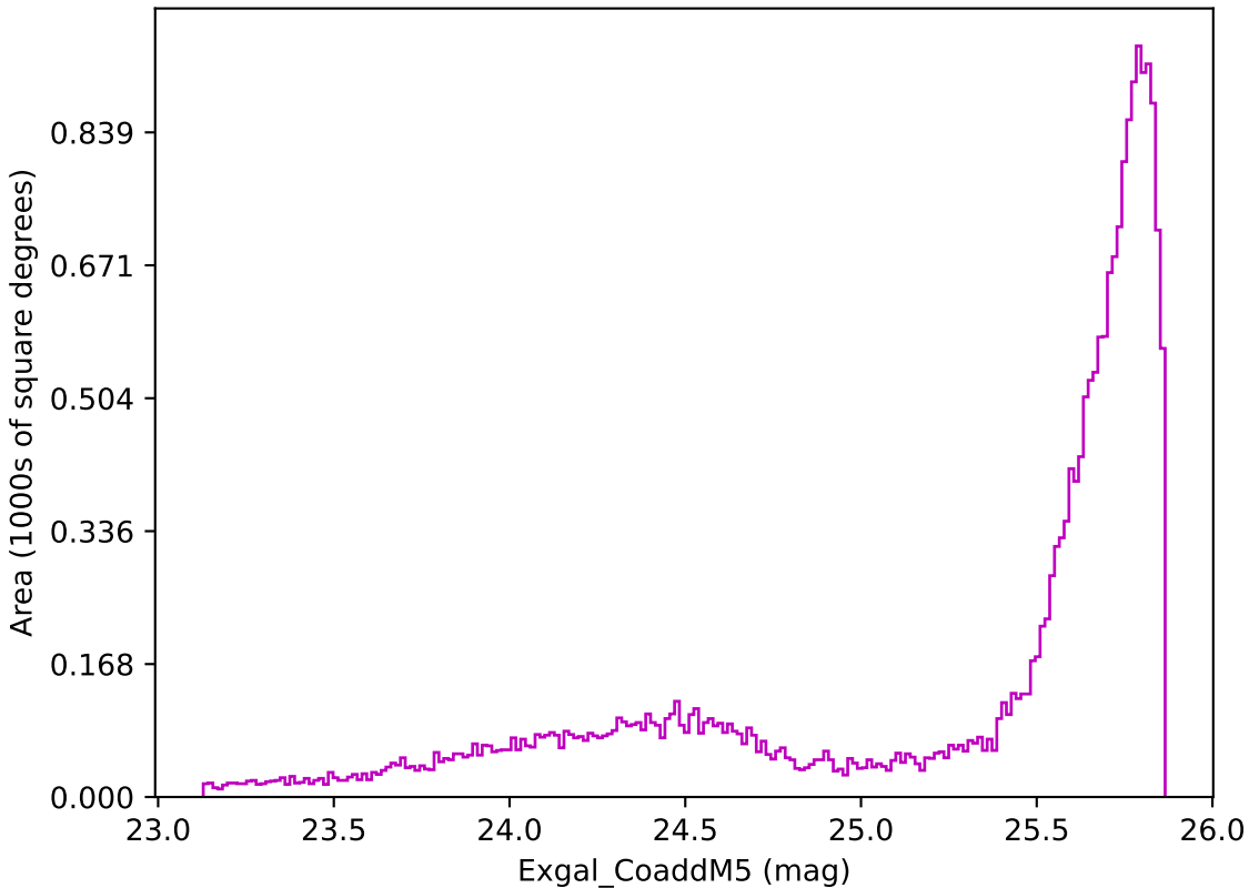
weather_cloudso8v3.4_10yrs All sky z band: Exgal_CoaddM5
