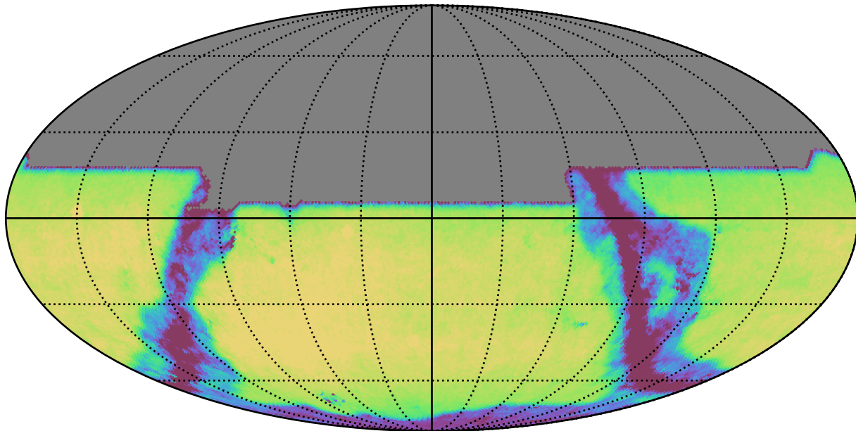
weather_cloudso8v3.4_10yrs All sky y band: Exgal_CoaddM5
