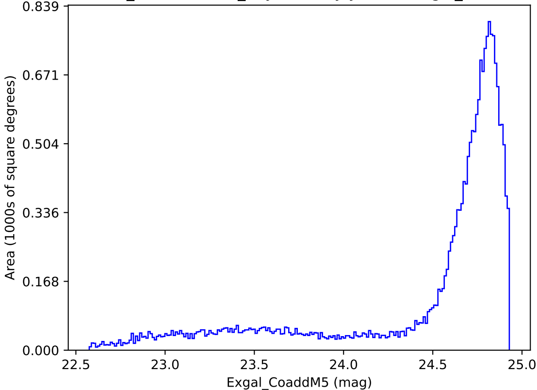
weather_cloudso8v3.4_10yrs All sky y band: Exgal_CoaddM5
