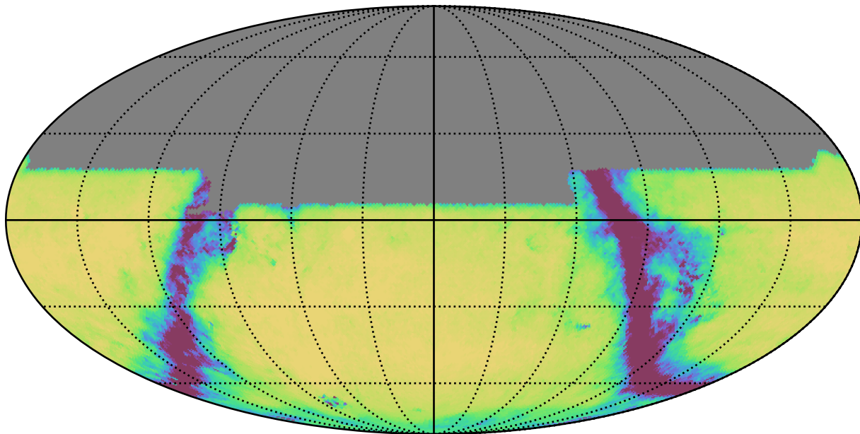
weather_cloudso8v3.4_10yrs All sky u band: Exgal_CoaddM5
