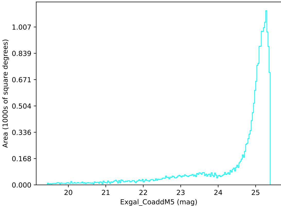
weather_cloudso8v3.4_10yrs All sky u band: Exgal_CoaddM5
