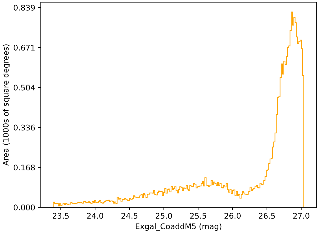
weather_cloudso8v3.4_10yrs All sky r band: Exgal_CoaddM5
