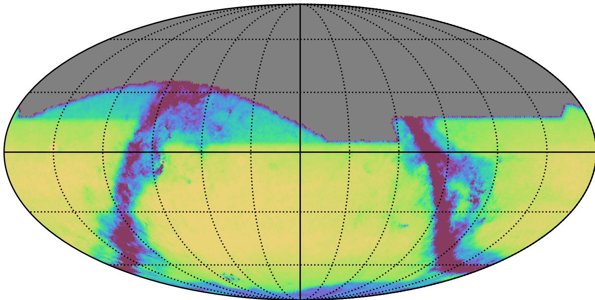
weather_cloudso8v3.4_10yrs All sky i band: Exgal_CoaddM5
