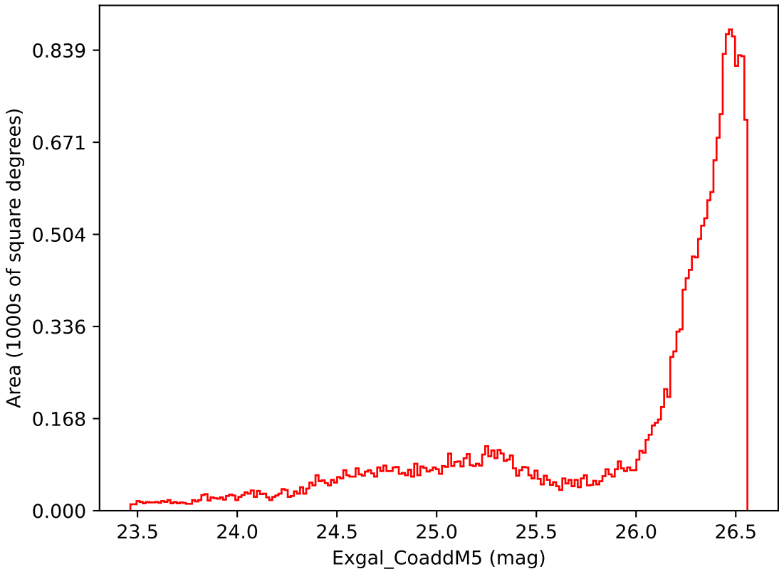
weather_cloudso8v3.4_10yrs All sky i band: Exgal_CoaddM5
