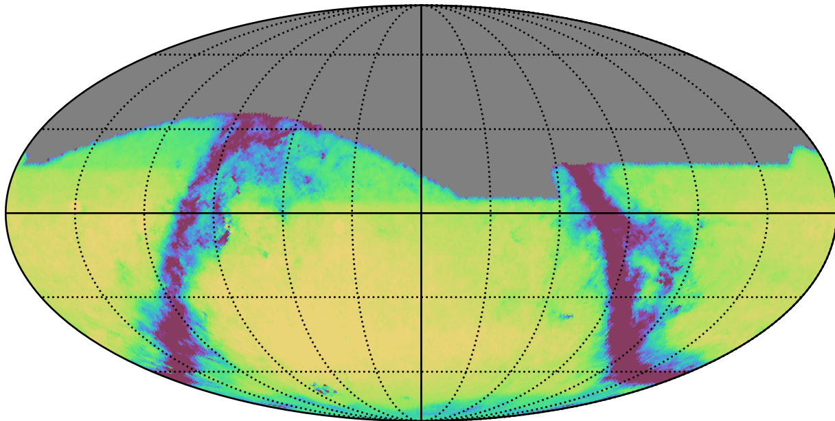
weather_cloudso8v3.4_10yrs All sky g band: Exgal_CoaddM5
