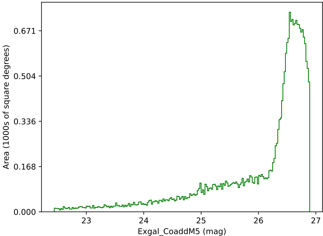
weather_cloudso8v3.4_10yrs All sky g band: Exgal_CoaddM5
