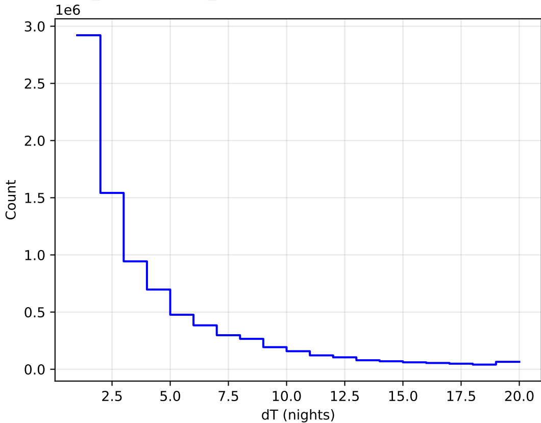
weather_cloudso8v3.4_10yrs WFD all bands: DeltaNight Histogram
