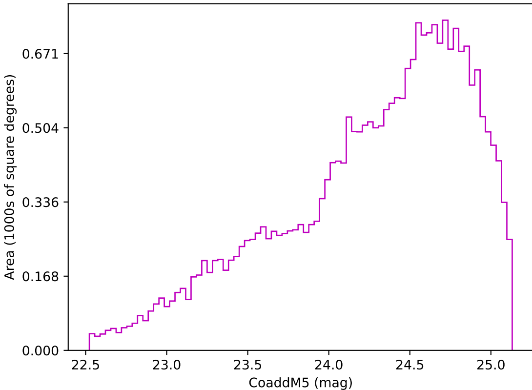
weather_cloudso8v3.4_10yrs Yr 3-4 z band: CoaddM5
