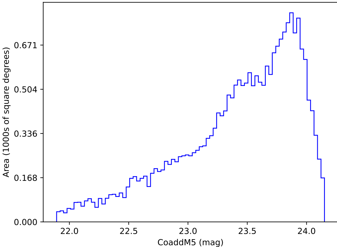
weather_cloudso8v3.4_10yrs Yr 3-4 y band: CoaddM5
