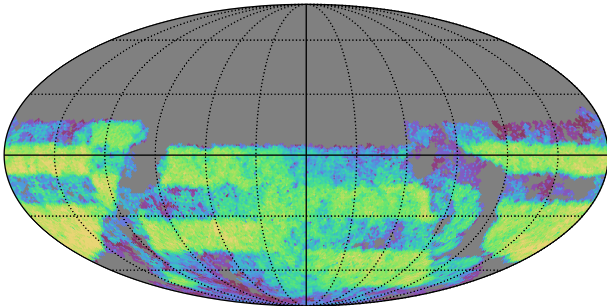
weather_cloudso8v3.4_10yrs Yr 3-4 u band: CoaddM5
