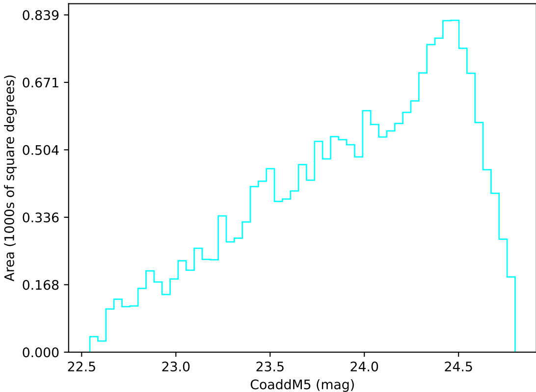
weather_cloudso8v3.4_10yrs Yr 3-4 u band: CoaddM5
