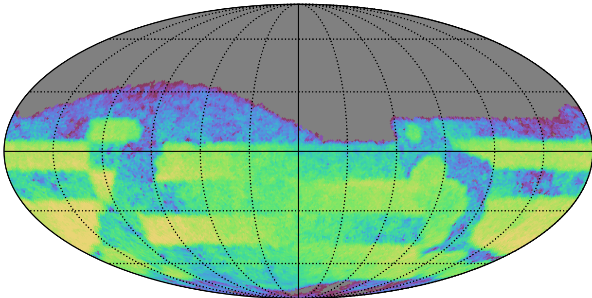
weather_cloudso8v3.4_10yrs Yr 3-4 r band: CoaddM5
