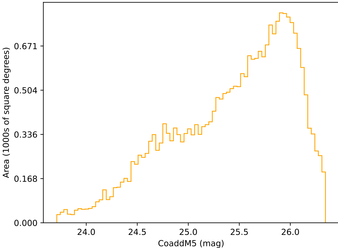
weather_cloudso8v3.4_10yrs Yr 3-4 r band: CoaddM5
