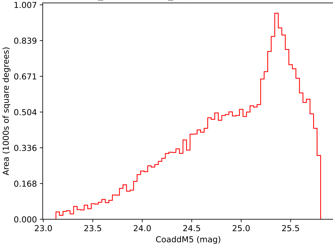
weather_cloudso8v3.4_10yrs Yr 3-4 i band: CoaddM5
