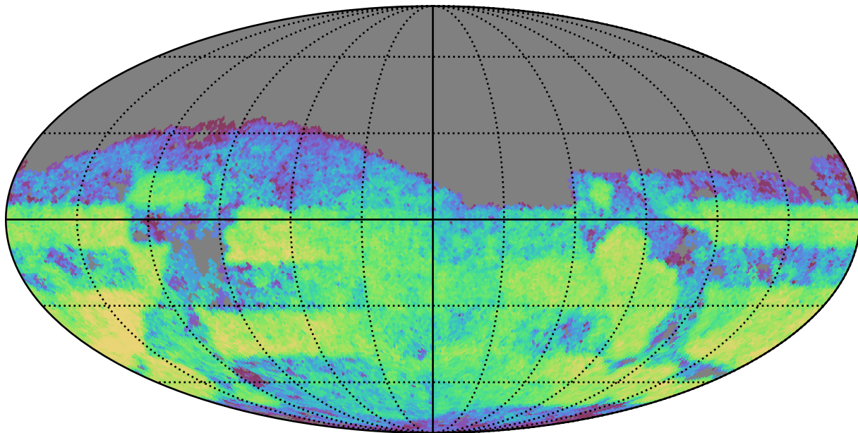
weather_cloudso8v3.4_10yrs Yr 3-4 g band: CoaddM5
