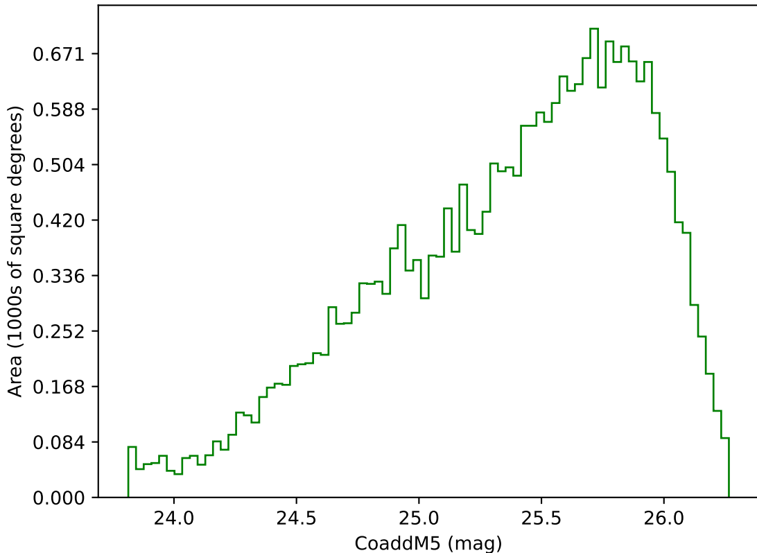
weather_cloudso8v3.4_10yrs Yr 3-4 g band: CoaddM5
