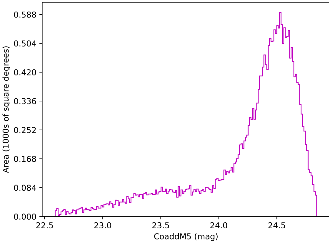
weather_cloudso8v3.4_10yrs Yr 1 z band: CoaddM5
