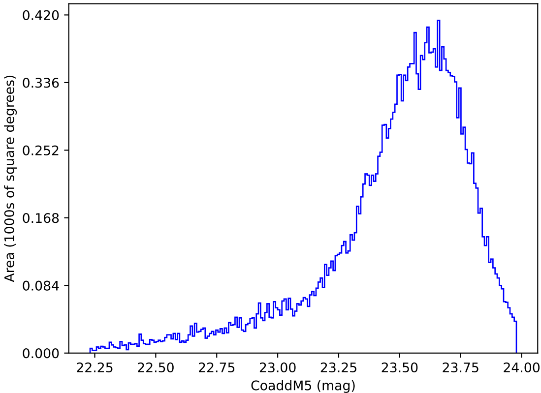
weather_cloudso8v3.4_10yrs Yr 1 y band: CoaddM5
