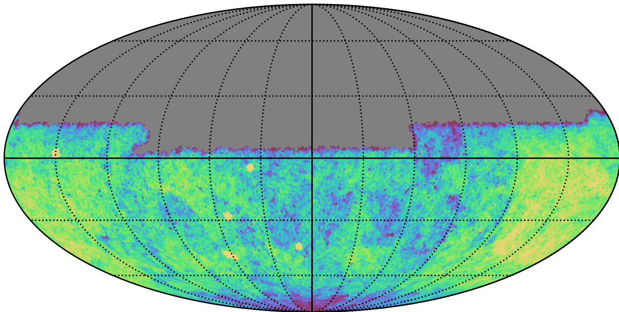
weather_cloudso8v3.4_10yrs Yr 1 u band: CoaddM5
