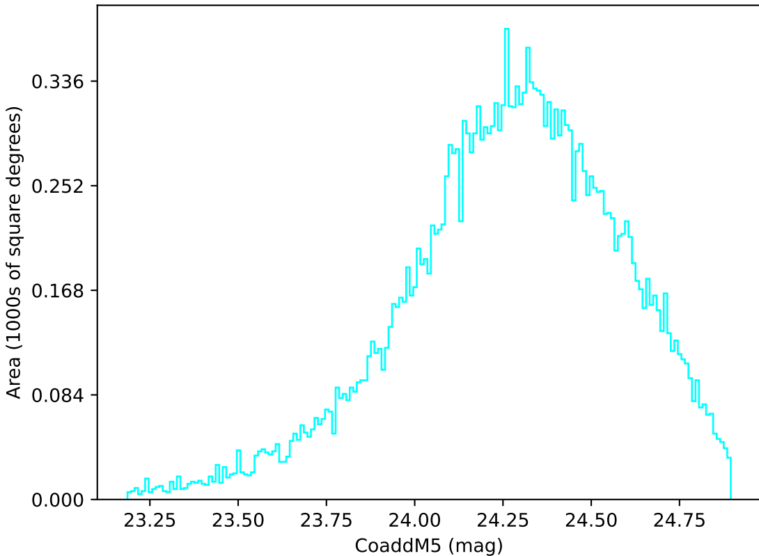
weather_cloudso8v3.4_10yrs Yr 1 u band: CoaddM5
