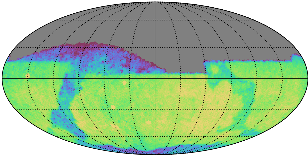
weather_cloudso8v3.4_10yrs Yr 1 i band: CoaddM5
