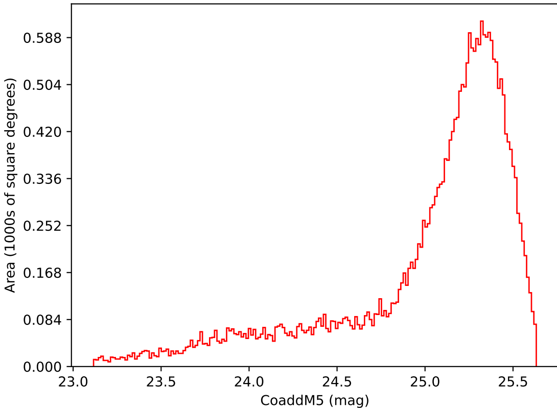
weather_cloudso8v3.4_10yrs Yr 1 i band: CoaddM5
