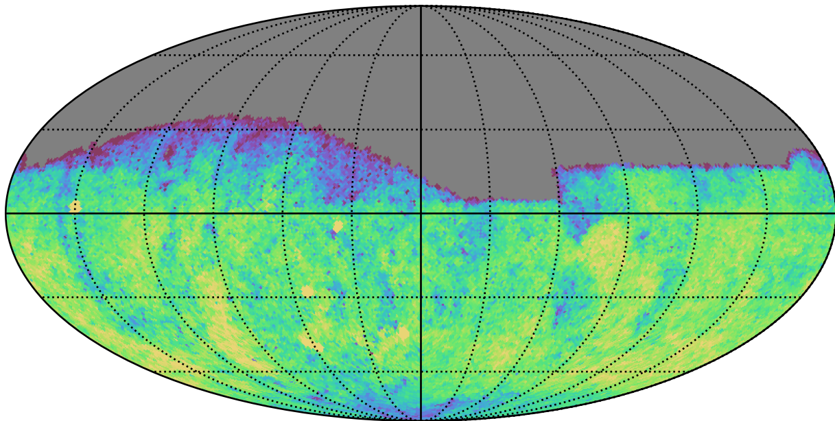
weather_cloudso8v3.4_10yrs Yr 1 g band: CoaddM5
