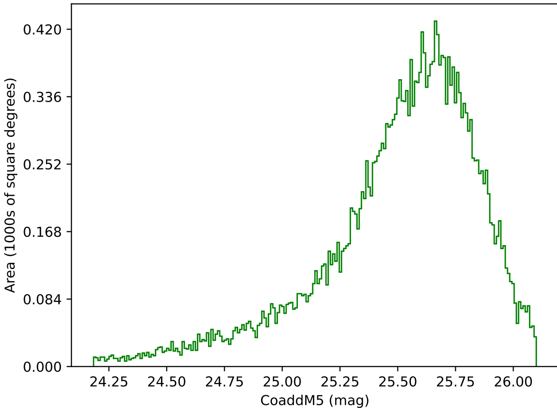
weather_cloudso8v3.4_10yrs Yr 1 g band: CoaddM5
