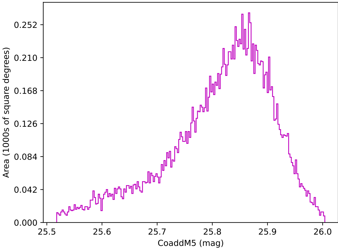
weather_cloudso8v3.4_10yrs WFD z band: CoaddM5
