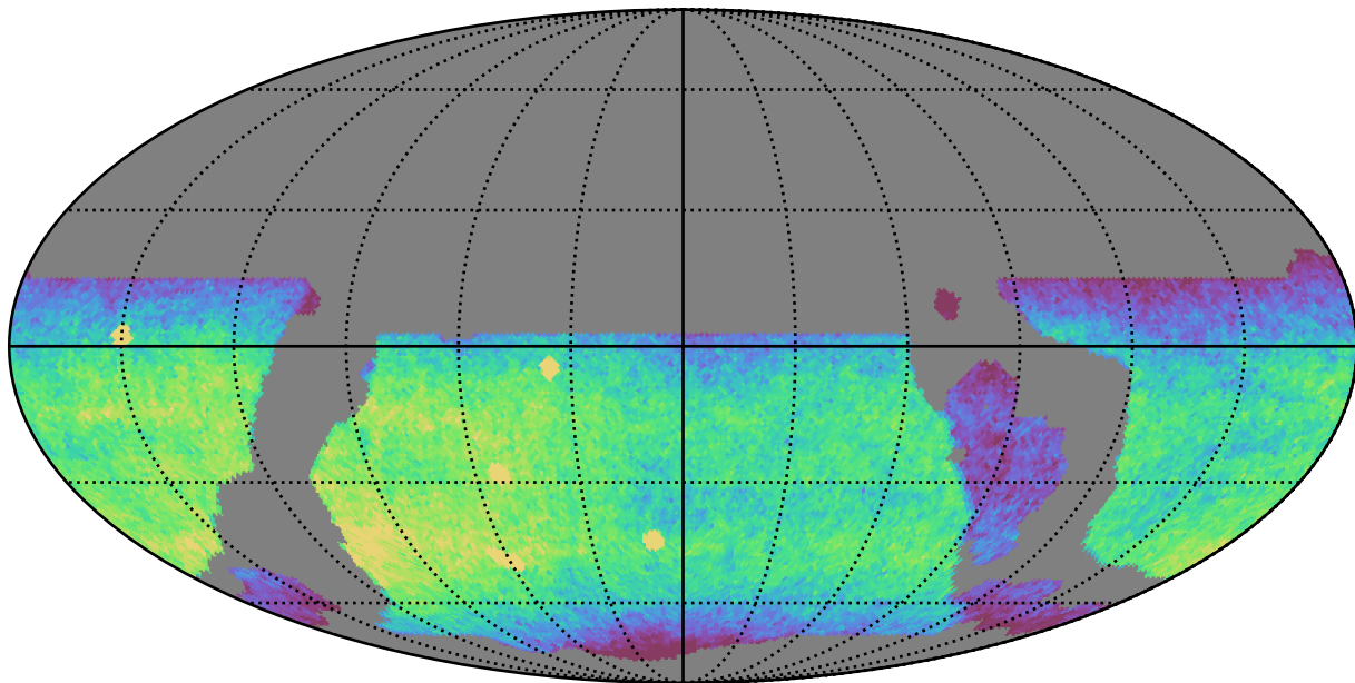
weather_cloudso8v3.4_10yrs WFD y band: CoaddM5
