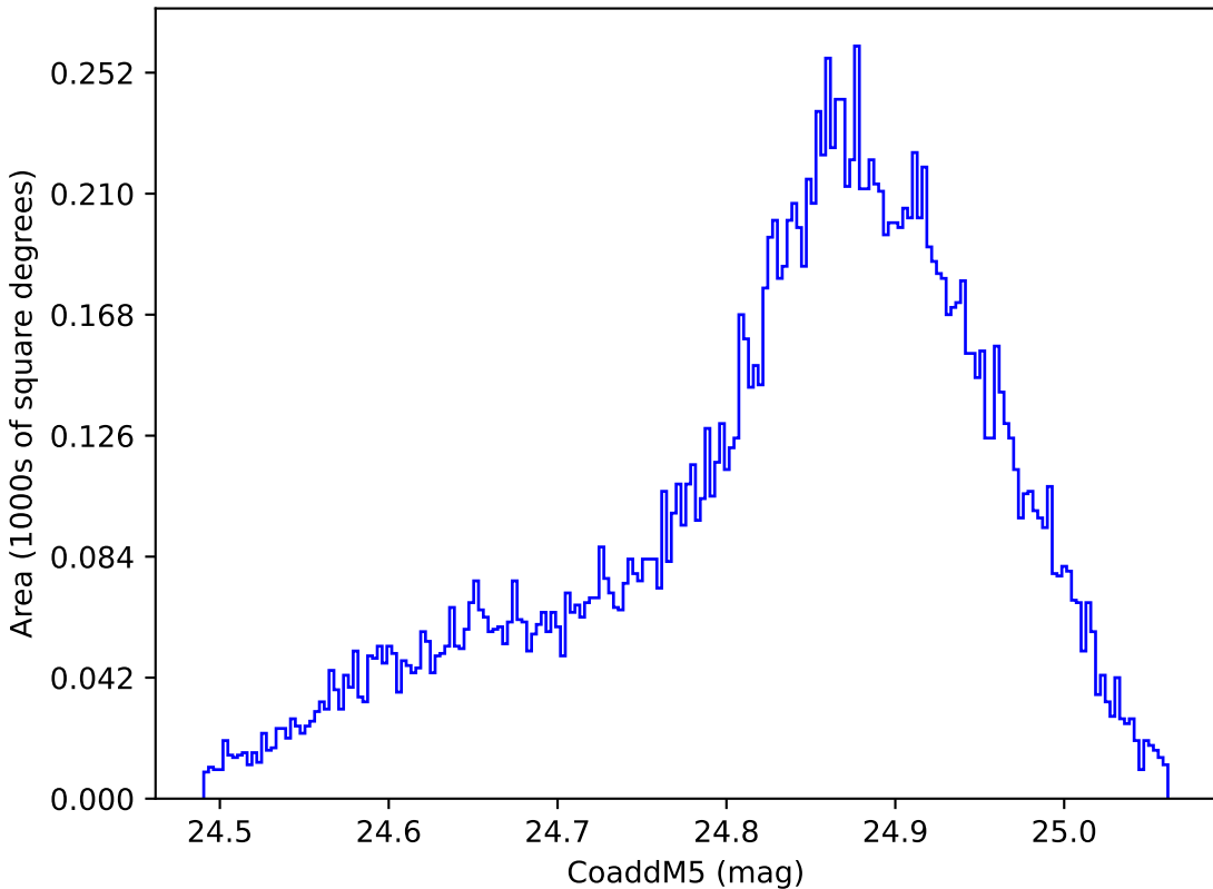
weather_cloudso8v3.4_10yrs WFD y band: CoaddM5
