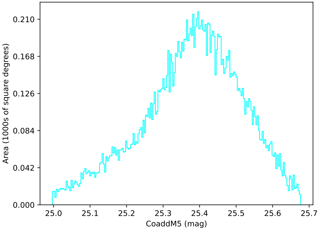
weather_cloudso8v3.4_10yrs WFD u band: CoaddM5
