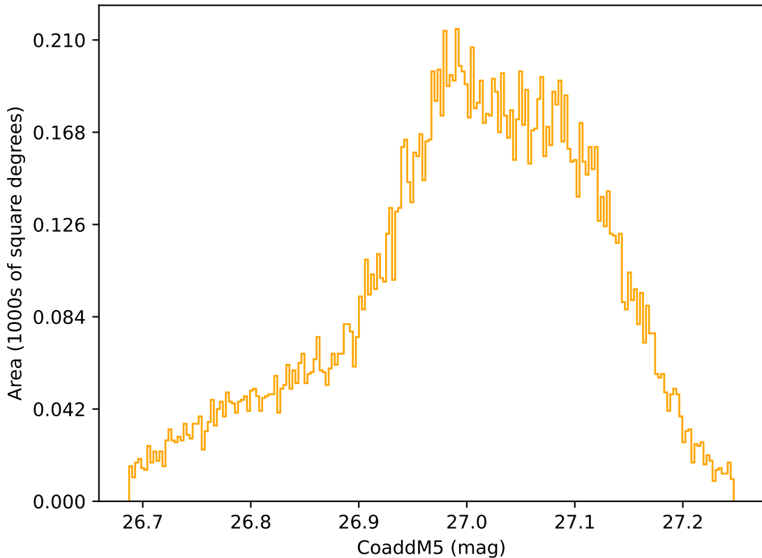
weather_cloudso8v3.4_10yrs WFD r band: CoaddM5
