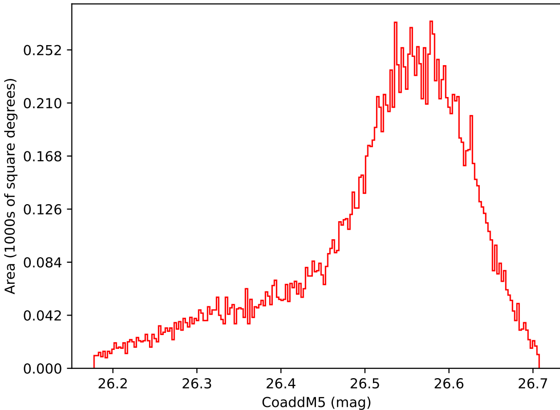
weather_cloudso8v3.4_10yrs WFD i band: CoaddM5
