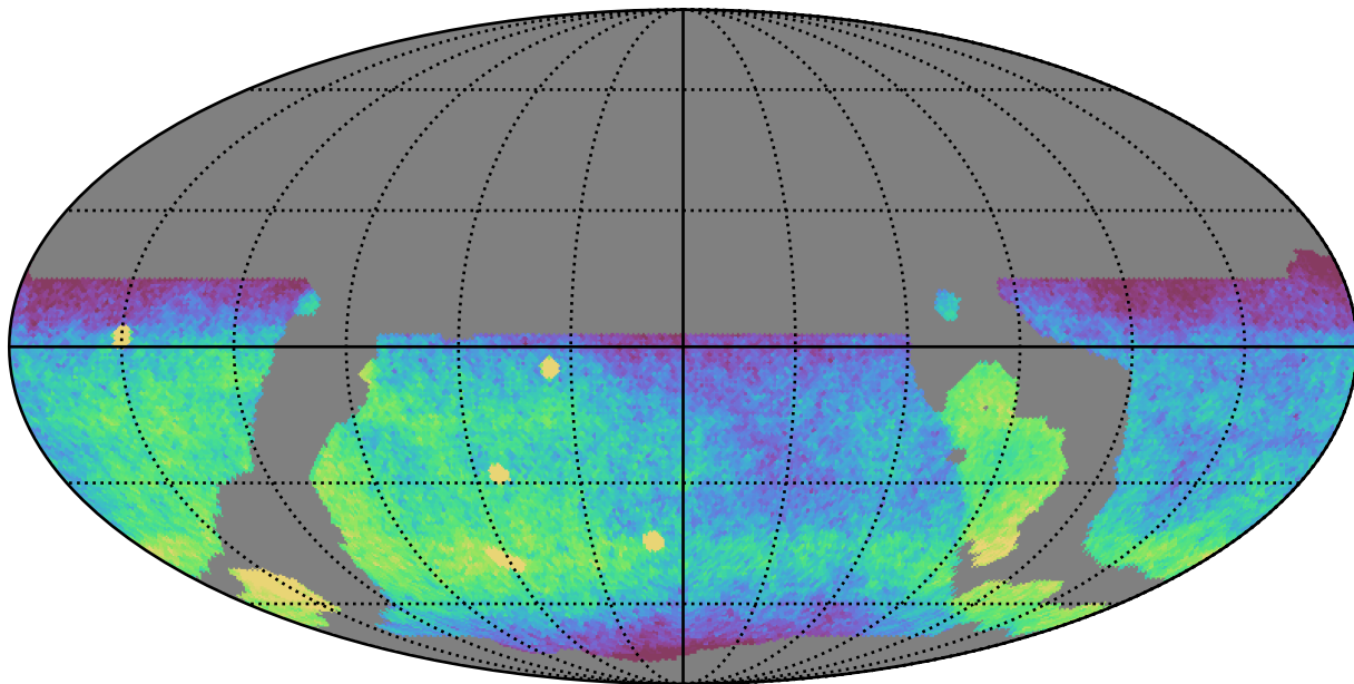
weather_cloudso8v3.4_10yrs WFD g band: CoaddM5
