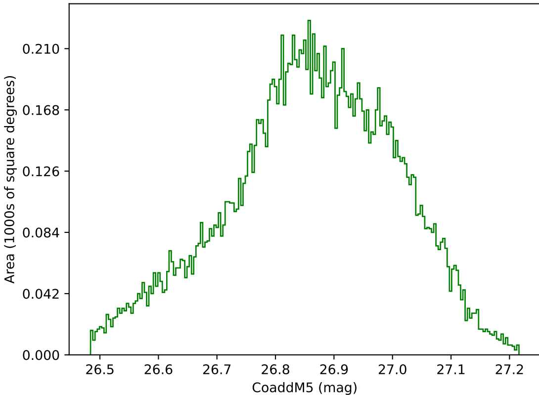
weather_cloudso8v3.4_10yrs WFD g band: CoaddM5
