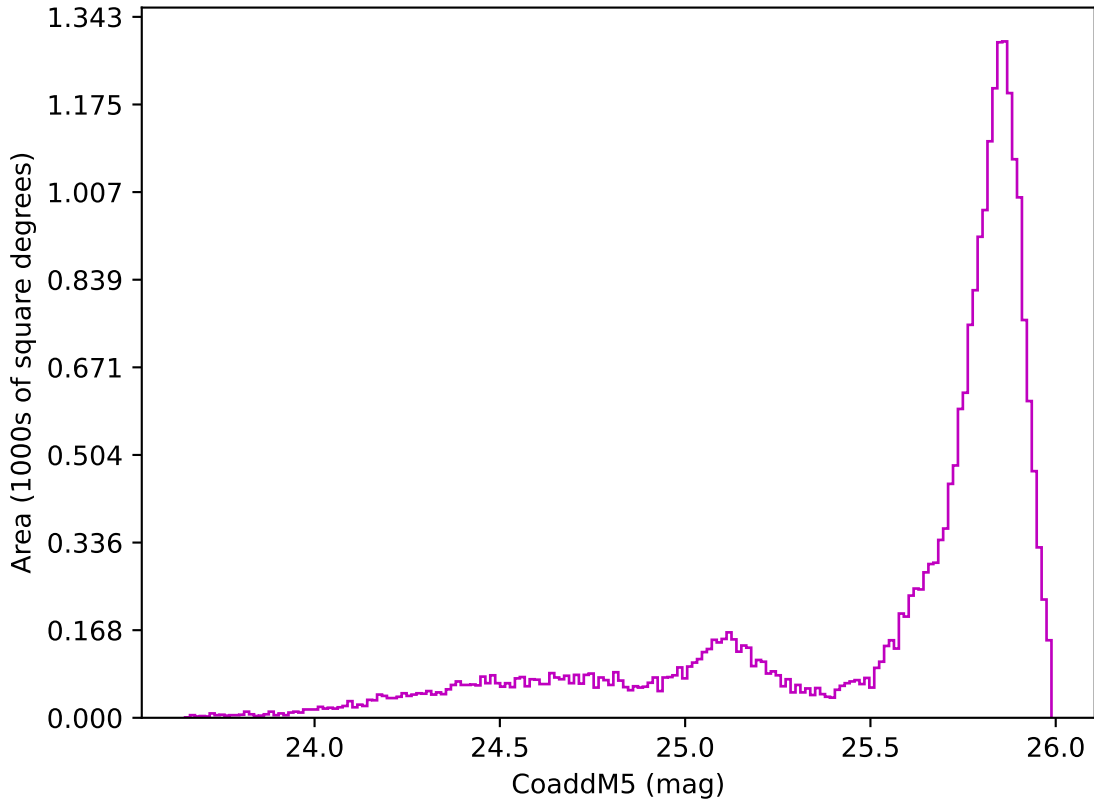
weather_cloudso8v3.4_10yrs All sky z band: CoaddM5
