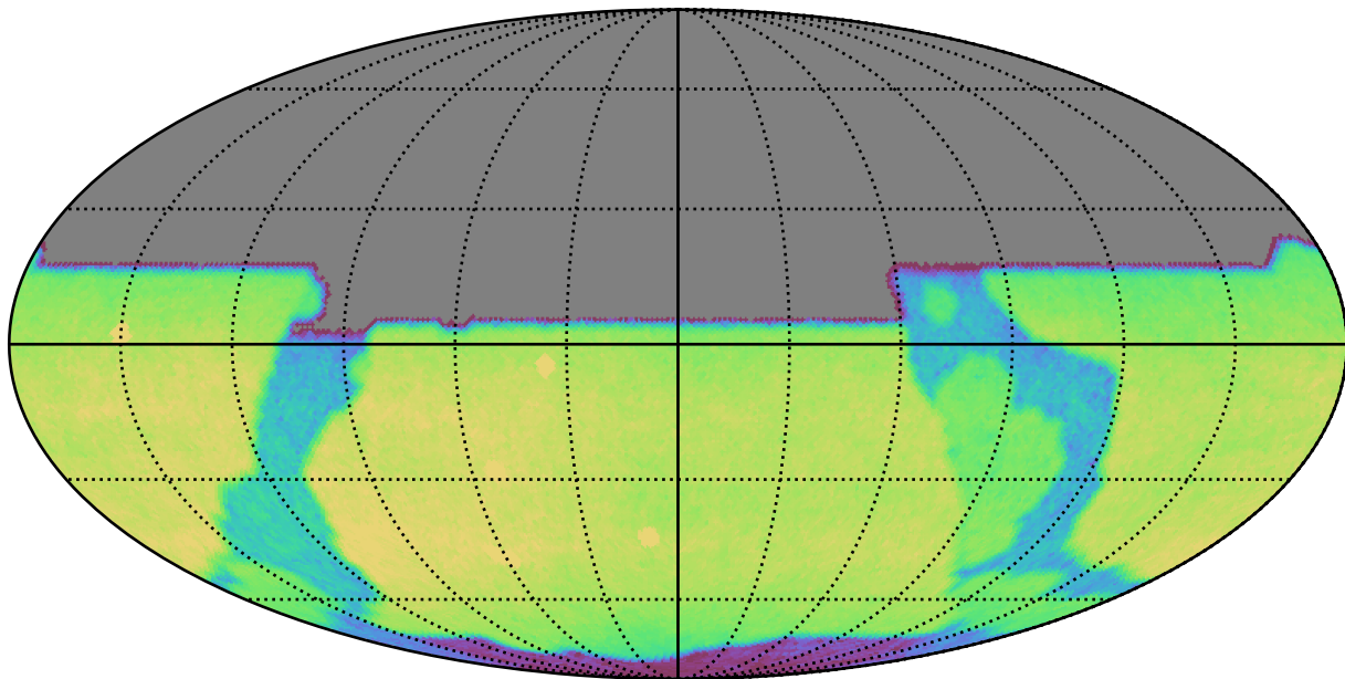
weather_cloudso8v3.4_10yrs All sky y band: CoaddM5
