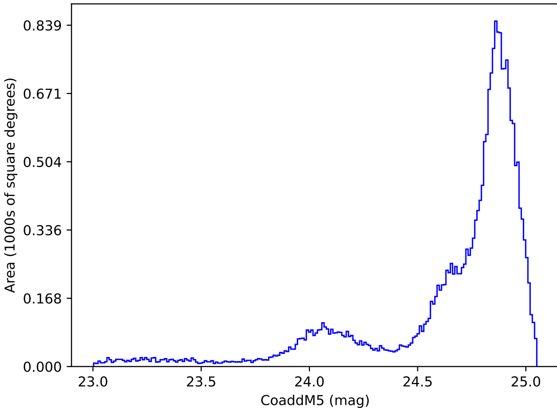
weather_cloudso8v3.4_10yrs All sky y band: CoaddM5
