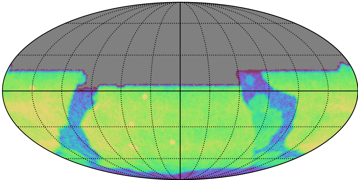
weather_cloudso8v3.4_10yrs All sky u band: CoaddM5
