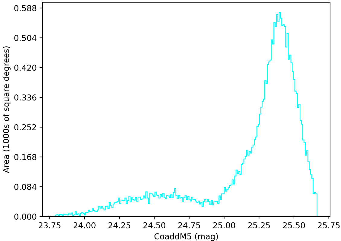
weather_cloudso8v3.4_10yrs All sky u band: CoaddM5
