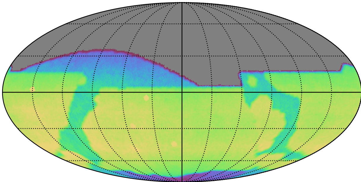
weather_cloudso8v3.4_10yrs All sky r band: CoaddM5
