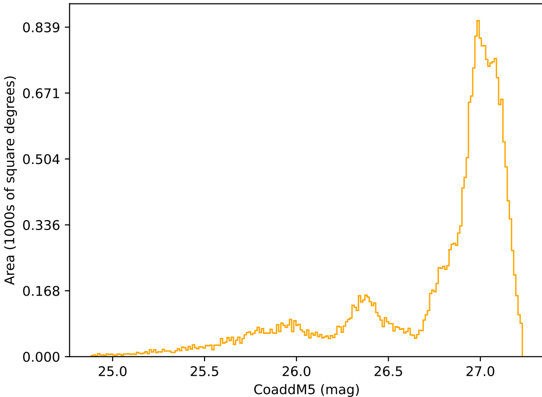
weather_cloudso8v3.4_10yrs All sky r band: CoaddM5
