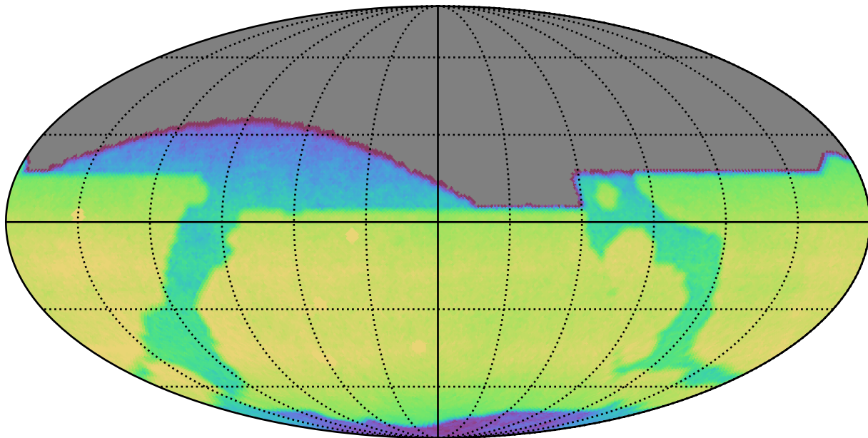
weather_cloudso8v3.4_10yrs All sky i band: CoaddM5
