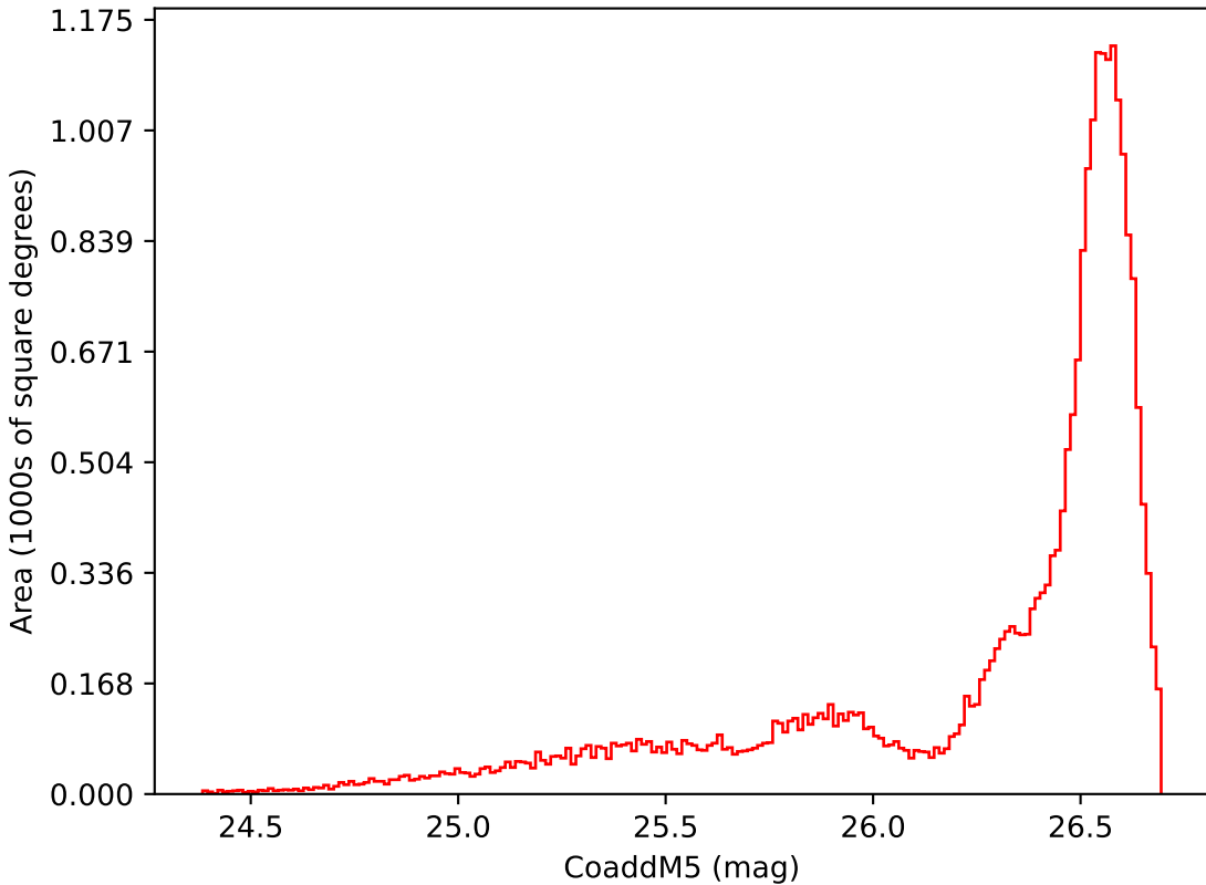
weather_cloudso8v3.4_10yrs All sky i band: CoaddM5
