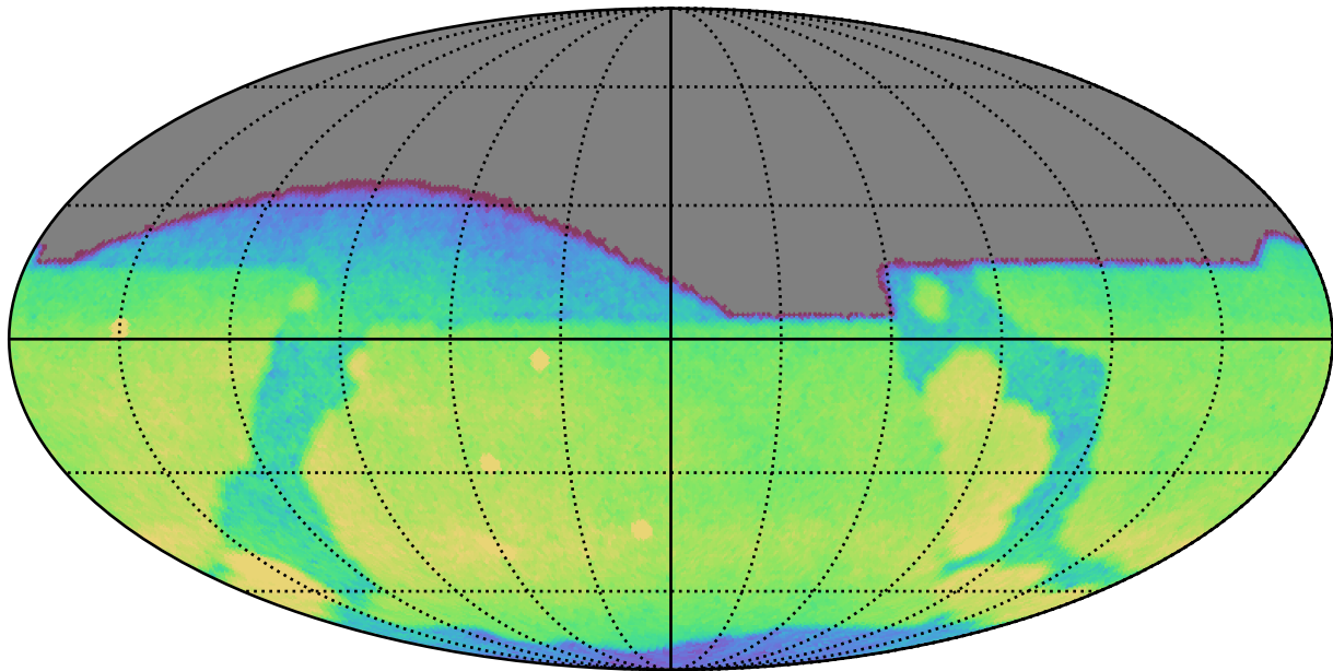
weather_cloudso8v3.4_10yrs All sky g band: CoaddM5
