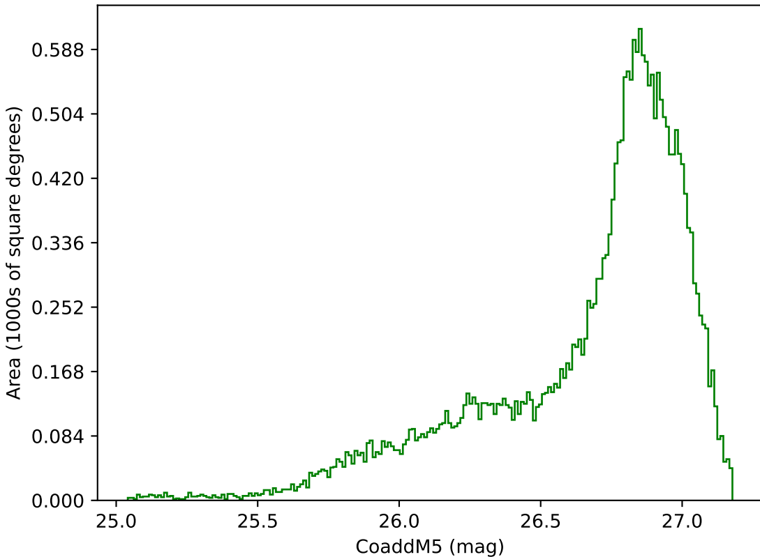
weather_cloudso8v3.4_10yrs All sky g band: CoaddM5
